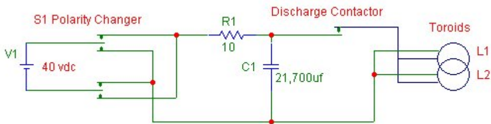
The Quadra test power supply
